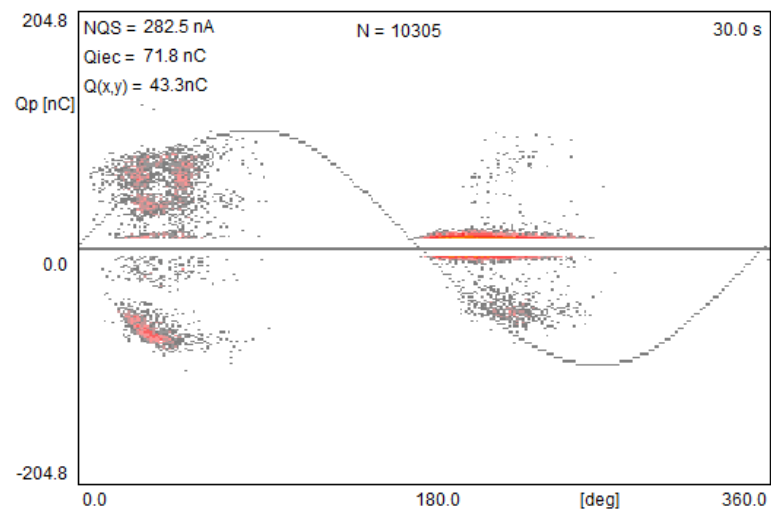
Figure 10: PD-pattern Phase W @ 7,0 kV, 100- 800 kHz
