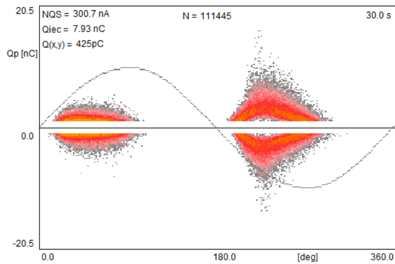
Figure 9: PD-pattern Phase W @ 4,2 kV, 100- 800 kHz
